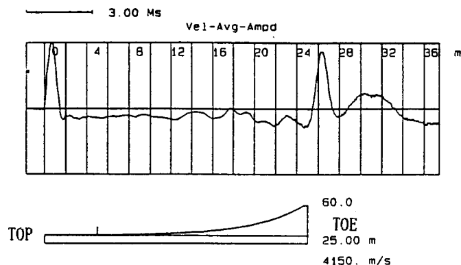
FIG. 3 Typical Velocity Record Indicating Pile of Generally Uniform Nature (Gradual Impedance Changes or Soil Friction)
