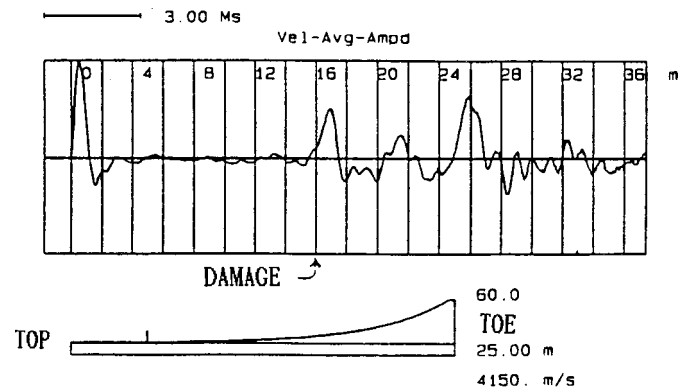
FIG. 4 Typical Velocity Record Indicating Major Changes in Impedance (Severe Damage or a Cracked Pile)
