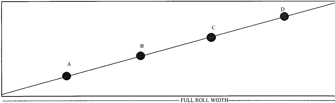
FIG. 2 Specimen Locations
